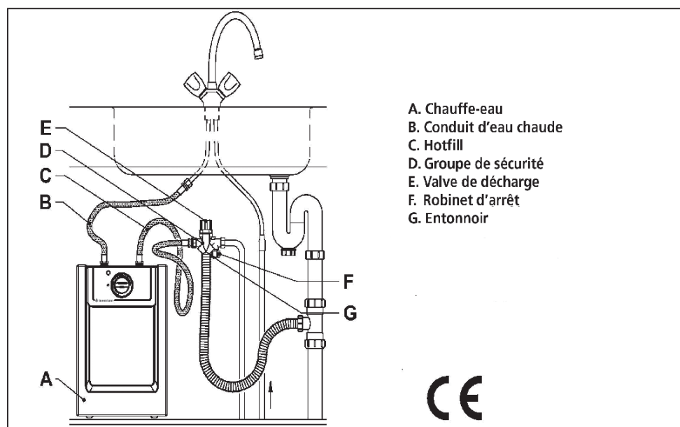
Fig. 5.2: Inventum Chauffe-eau Q10 'Hotfill'
